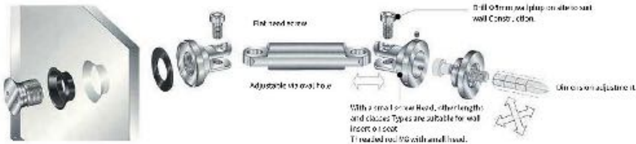
Components and assembly of the wall fixing
