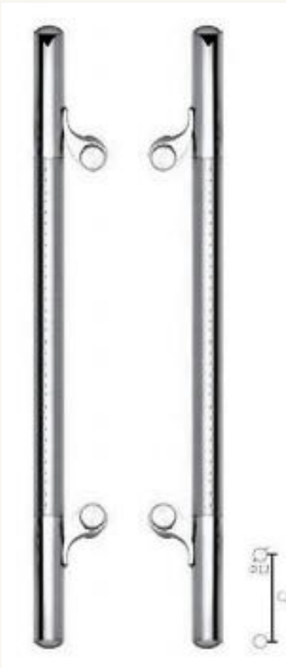
FINISHES / DIMENSIONS
