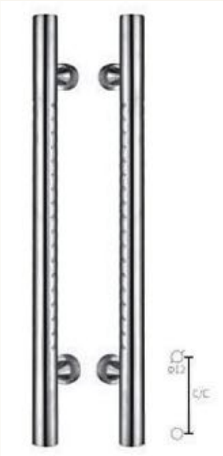
FINISHES / DIMENSIONS
